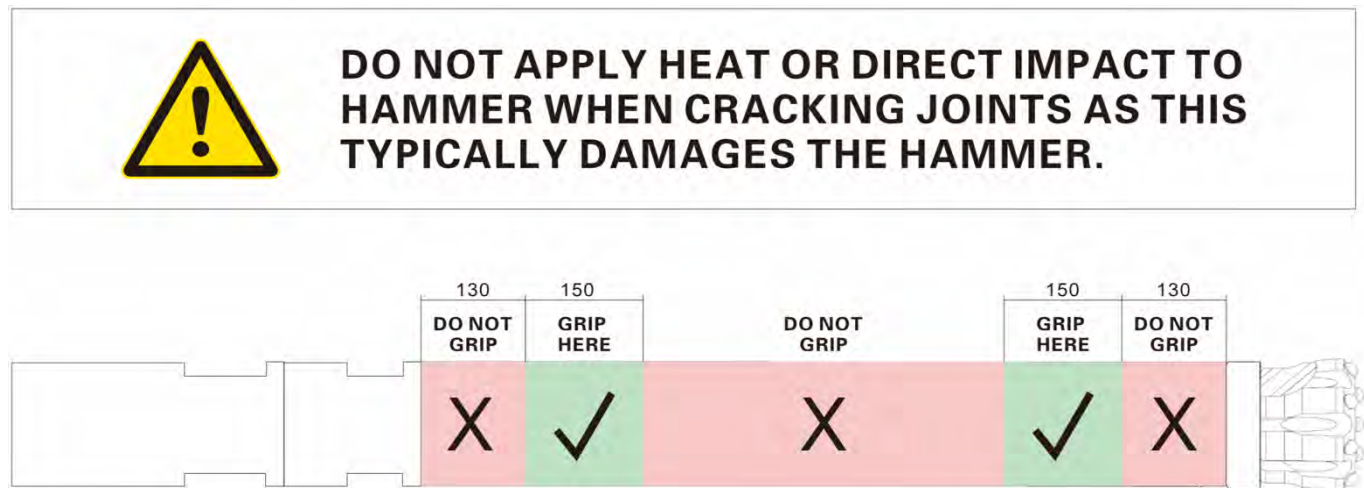
Figure 1: Gripping Locations for BD DRILL Reverse Circulation Hammer
